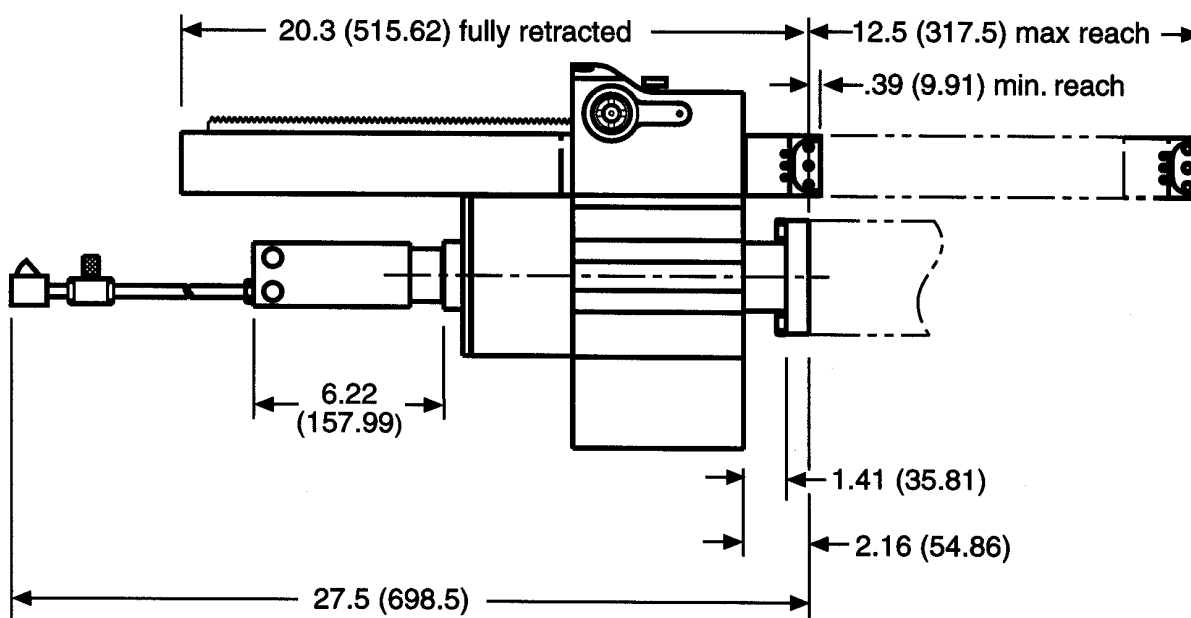
PL2000 with Pneumatic Motor
